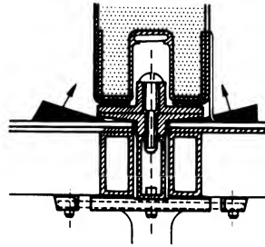
⑧ Floor/wall section: dividing wall
